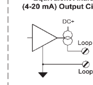
Equivalent Analog (4-20 mA) Output Circuit
