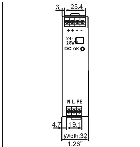
Fig. 20-1 Front view
